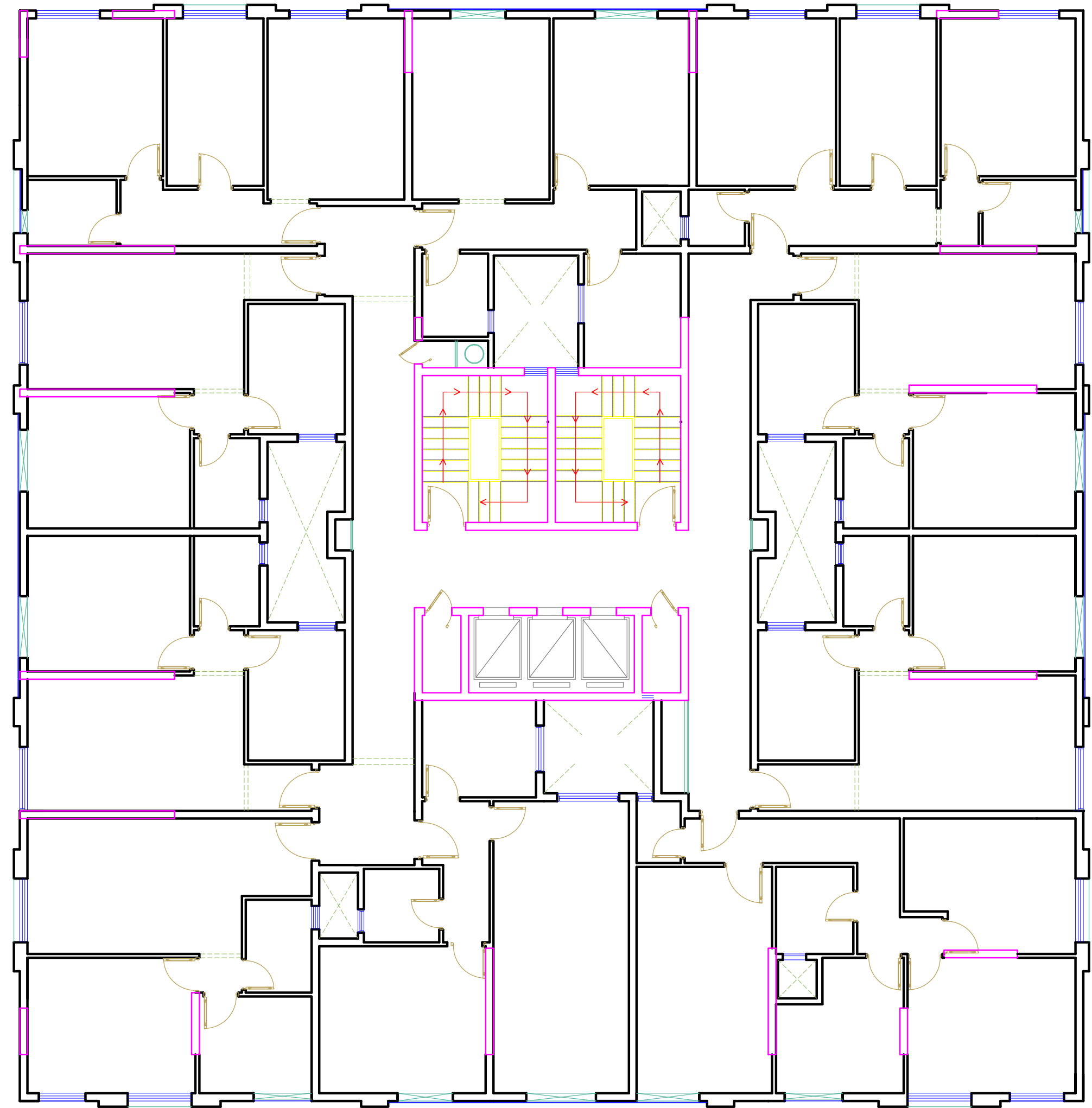
16th TO 19th TYP.FLOOR PLAN
