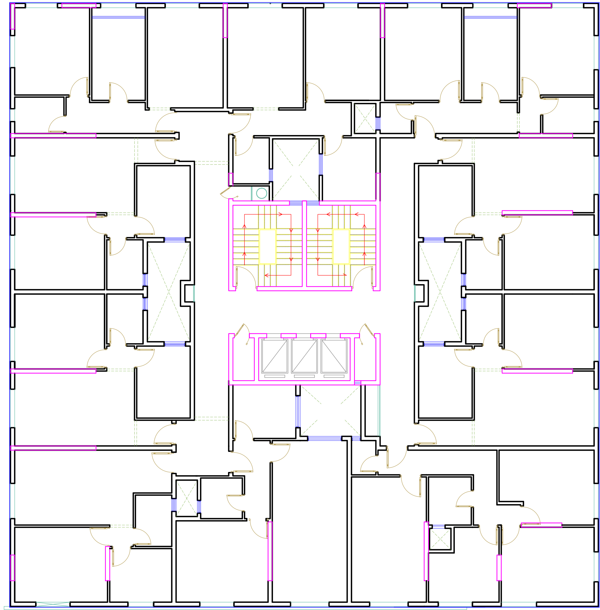
4thTYPICAL FLOOR PLAN
