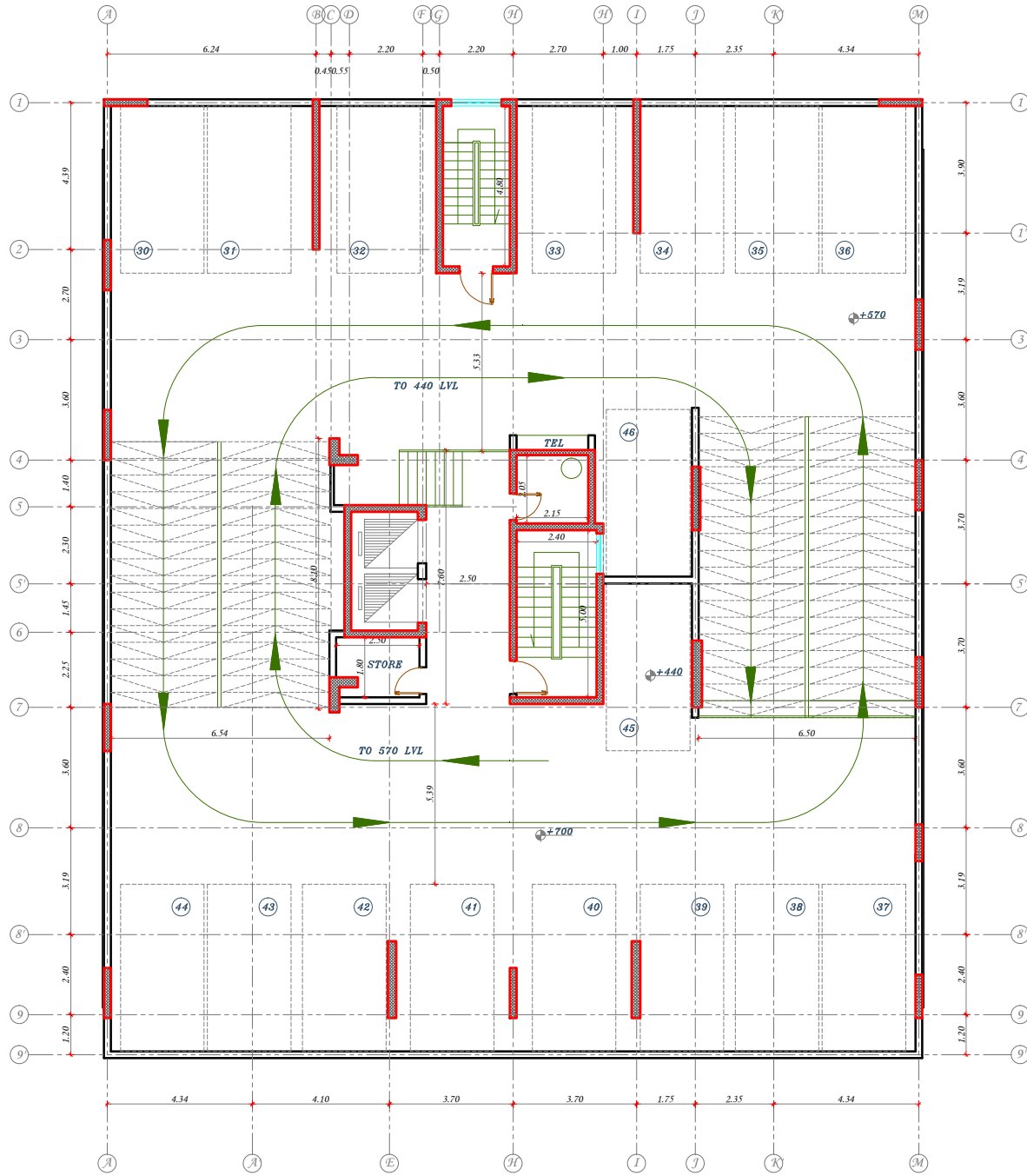
SECOND PARKING FLOOR
